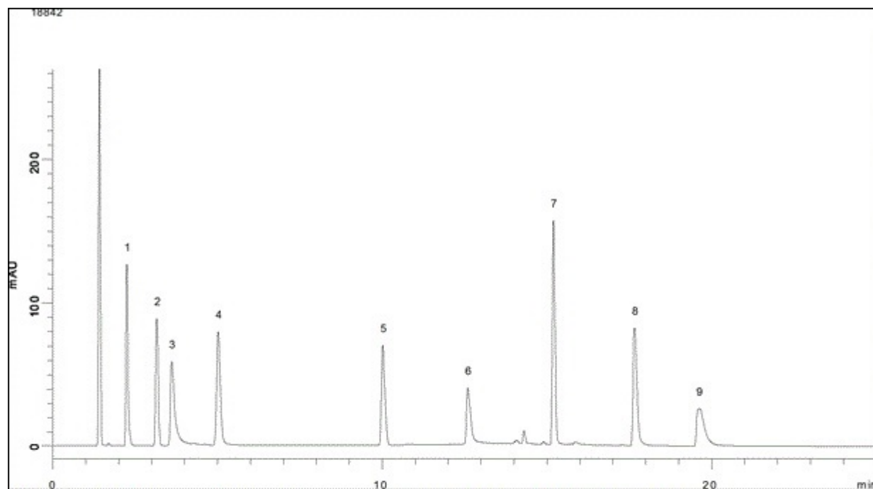
Figure 2: Water-soluble vitamins on Kinetex 2.6 um HILIC 150 x 4.6 mm.
