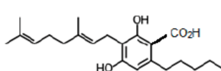
10. Cannabigerolic Acid (CBGA)
