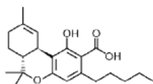
9. Tetrahydrocannabinolic Acid (THCA)
