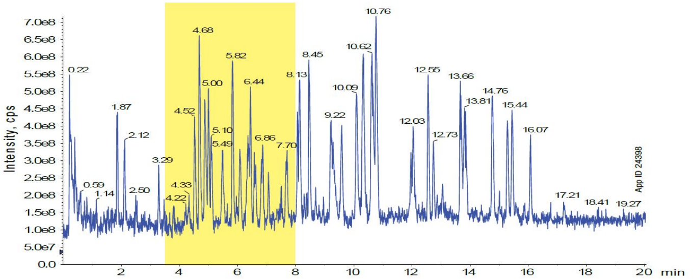
Figure 1 Waters® ACQUITY® BEH 1.7 µm C18; 420 Bar
